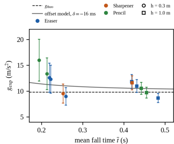
Fig. 1. Experimental g against mean fall time. Error bars: \sigma_g from Eq. (7) with the empirical \sigma_t = 24.5 ms. Dashed line: g_{\text{theo}} . Grey curve: Eq. (8) with g = g_{\text{theo}} and a constant offset \delta = -16 ms; it captures the rise of g_{\text{exp}} at short fall times.
