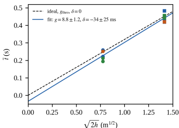
Fig. 2. Mean fall time against \sqrt{(2h)} . The free-fall line through the origin uses g_{\text{theo}} ; the solid line is a two-parameter fit whose slope gives g and whose intercept gives the timing offset \delta . Colours and symbols as in Fig. 1.
