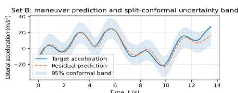
Fig. 1. Representative Set B target-maneuver prediction and 95% split-conformal band
