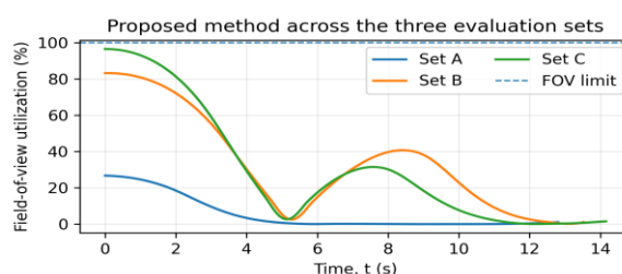
Fig. 3. Field-of-view utilization of the proposed method for Sets A, B, and C
