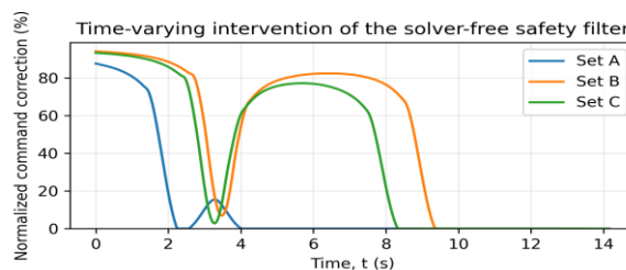
Fig. 4. Normalized time-varying correction applied by the solver-free safety filter in the three sets
