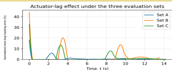
Fig. 5. Normalized inner-loop command-tracking error in the three sets
