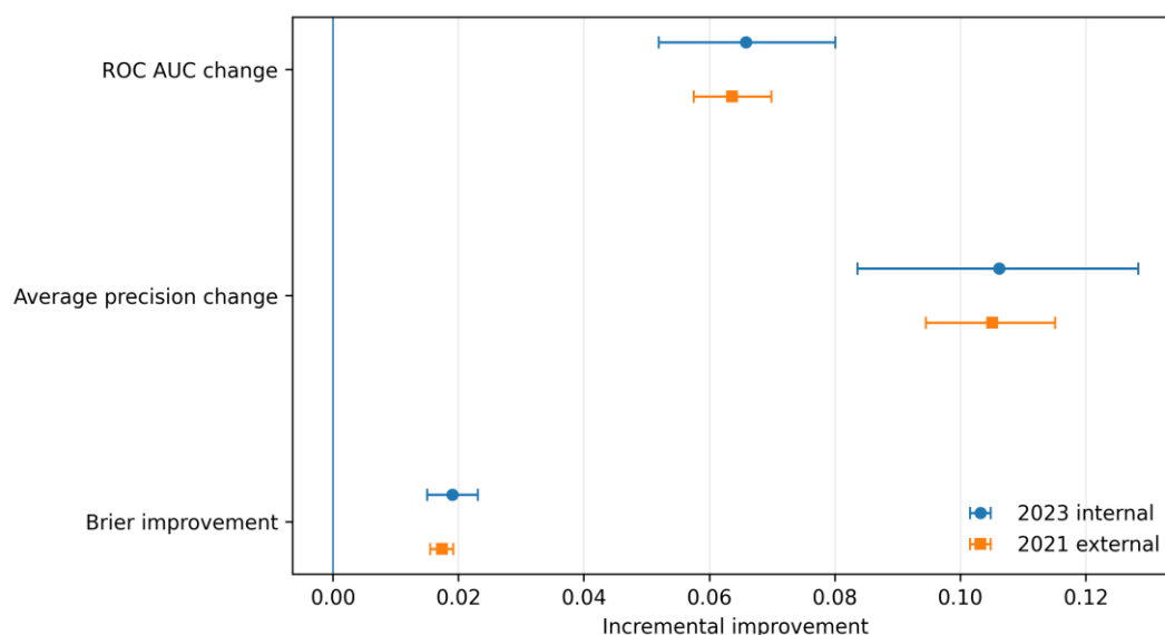
Fig. 2. Incremental feature-set improvements in the 2023 internal comparison and 2021 cross-wave external validation. Points show paired differences and bars show conditional 95% percentile bootstrap intervals. Brier improvement is baseline Brier minus expanded-model Brier.
