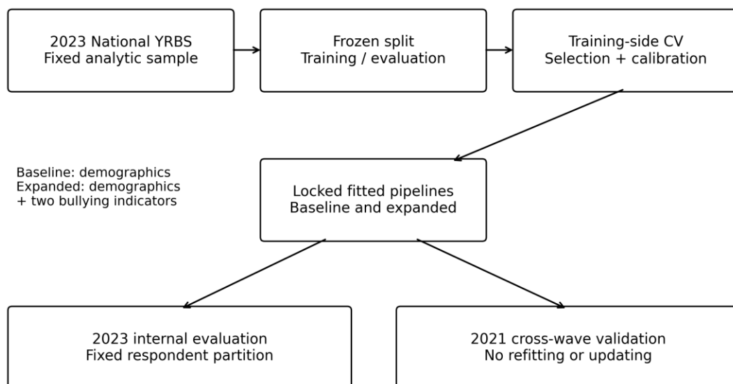
Fig. 1. Evaluation workflow. Calibration fitting uses training data only. The fixed pipelines are evaluated on the 2023 internal comparison set and the separate 2021 wave without external-wave tuning, preprocessing refit, or recalibration.
