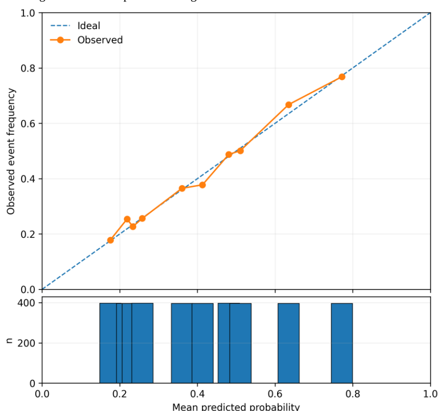
Fig. 3. Reliability diagram for the selected expanded HGB model with Platt scaling on the 2023 internal evaluation set. Ten equal-frequency bins show mean predicted probability and observed event frequency, with the lower panel showing the number of observations per bin.
